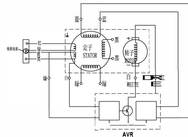
ALTERNATOR PRINCIPLE DRAWING
